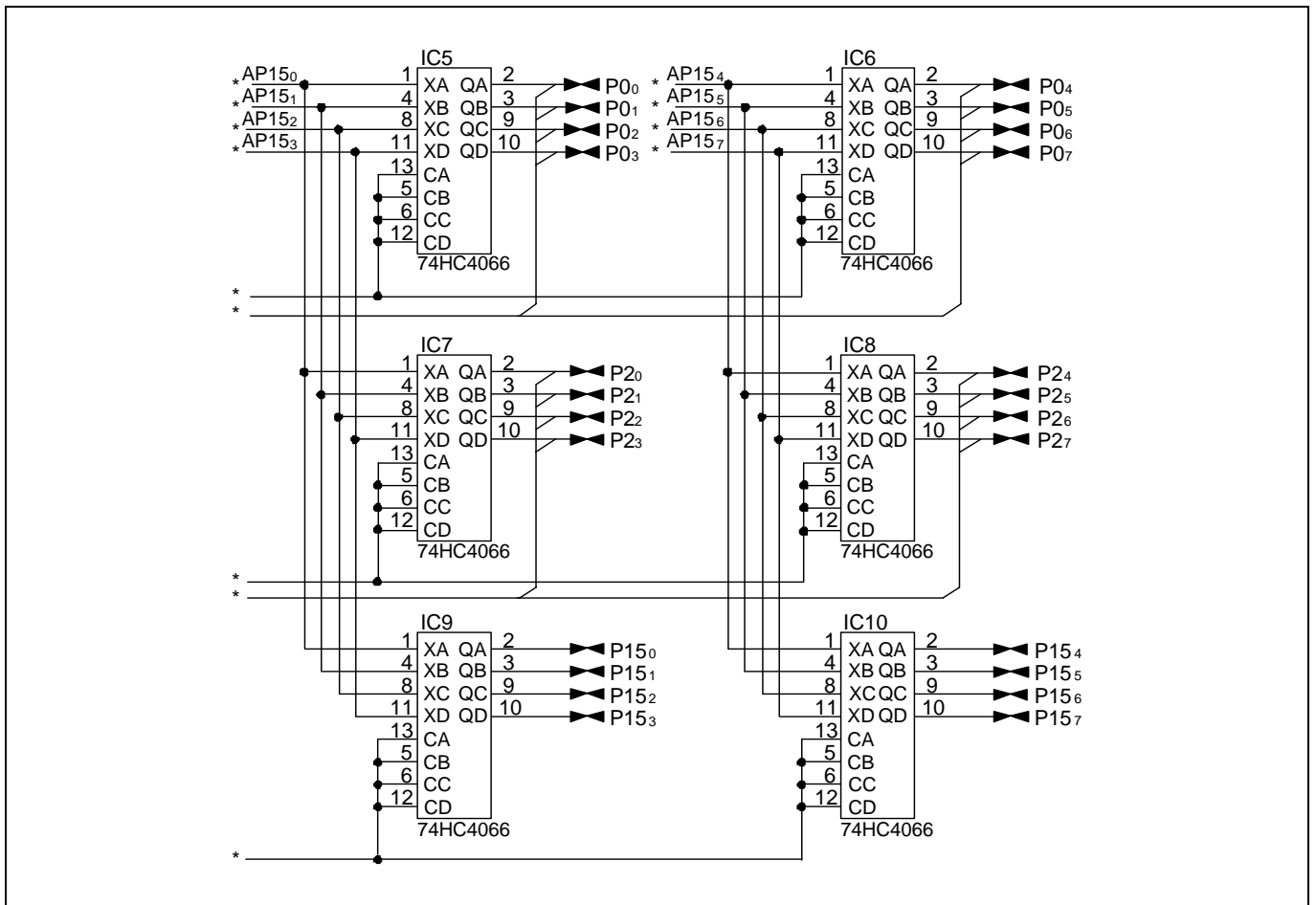
Figure 4.2 Connection diagram (2/2)
